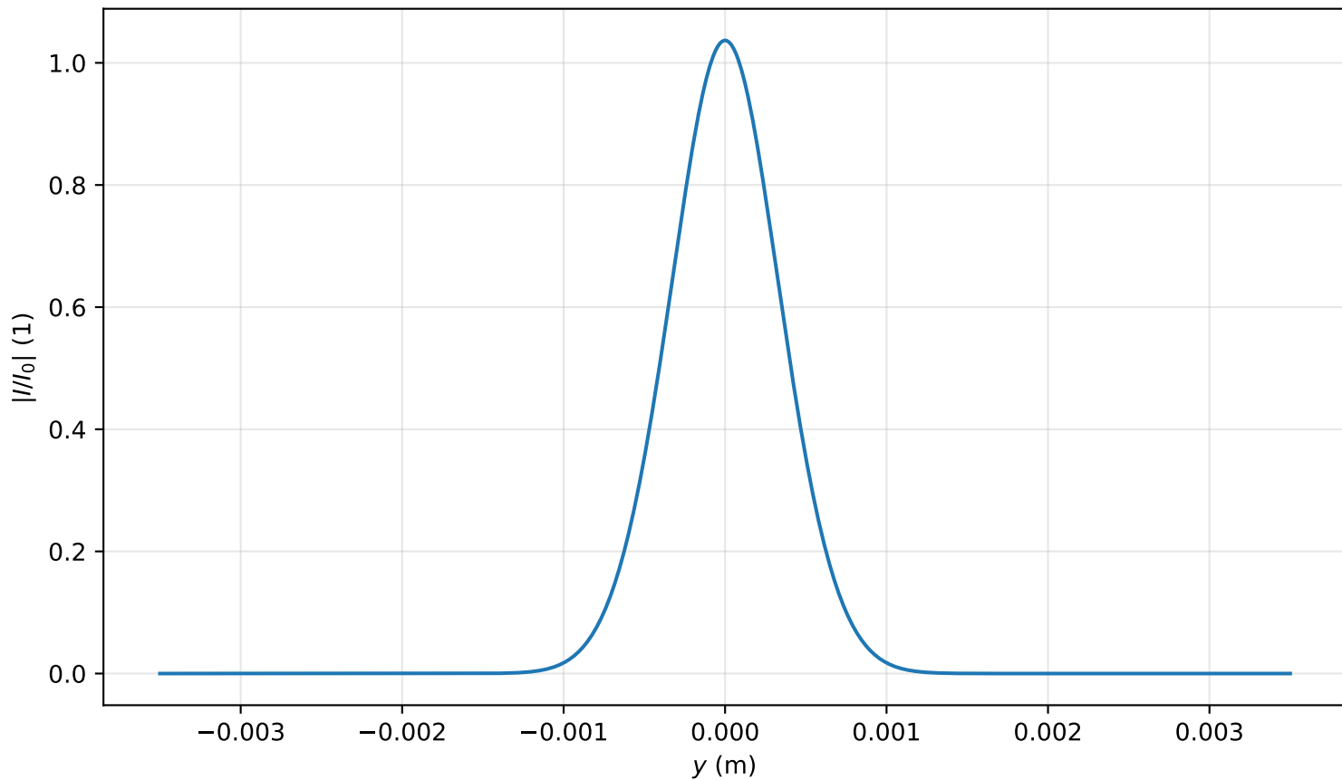
Intensity profile I(x=0, y, z=0.239)/I_0 , \text{Pin}=0.9\text{Pcr} , artificial time
